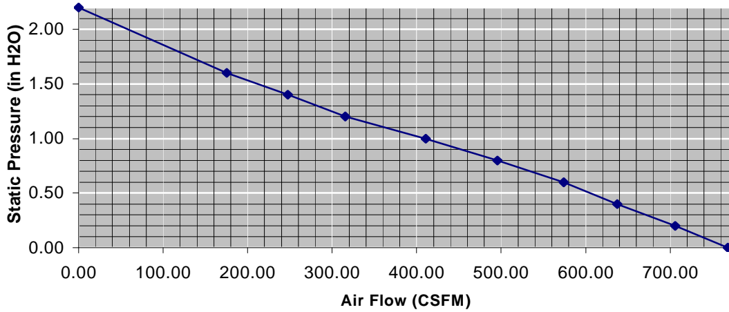
Air Flow Performance of the DB928-2430 Motorized Impeller
